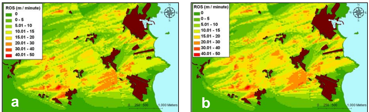
Figure 3 – Maximum values of rate of spread (ROS) for moderate (a) and severe (b) simulation scenarios (prevailing wind speed 6 \text{ m s}^{-1} ). Brown color indicates the urban areas.
