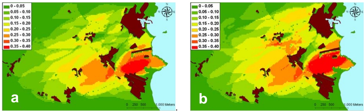
Figure 2 – Fire probability indexes for moderate (a) and severe (b) simulation scenarios (prevailing wind speed 6 \text{ m s}^{-1} ). Brown color indicates the urban areas.
