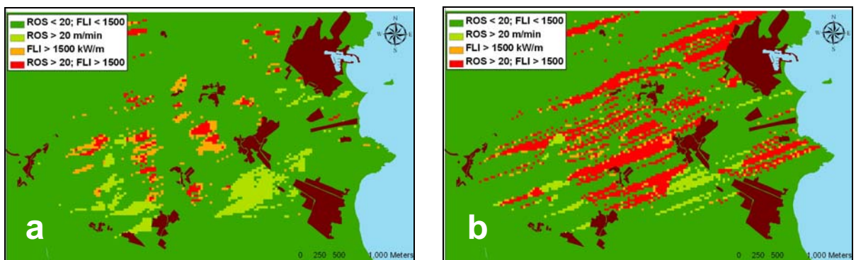
Figure 5 – Fire severity maps obtained using the severe scenario and two different wind conditions: wind speed 6 \text{ m s}^{-1} (a) and 10 \text{ m s}^{-1} (b). Brown color indicates the urban areas.
