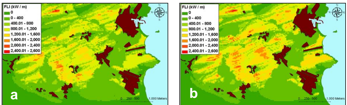
Figure 4 – Maximum values of fireline intensity (FLI) for moderate (a) and severe (b) simulation scenarios (prevailing wind speed 6 \text{ m s}^{-1} ). Brown color indicates the urban areas.
