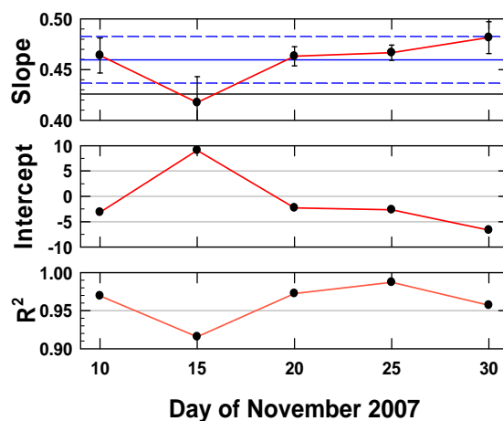
Fig. 5. Time series of slope, intercept, and R^2 for MTSAT 1R visible band using desert only.
