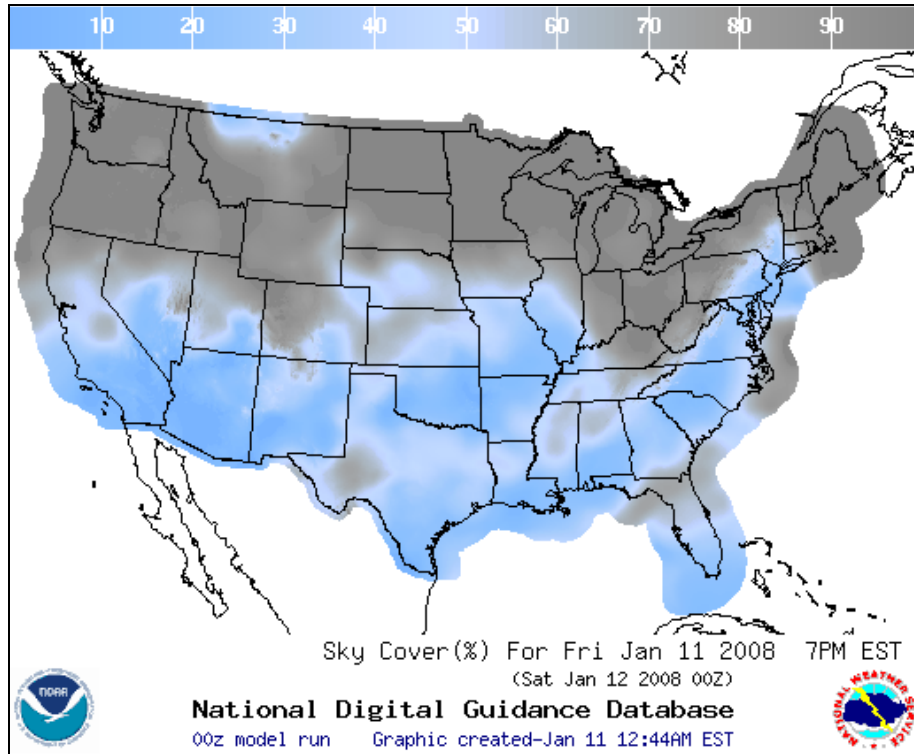
Figure 3. Gridded MOS sky cover guidance valid Jan 12, 2008, 0000 UTC
