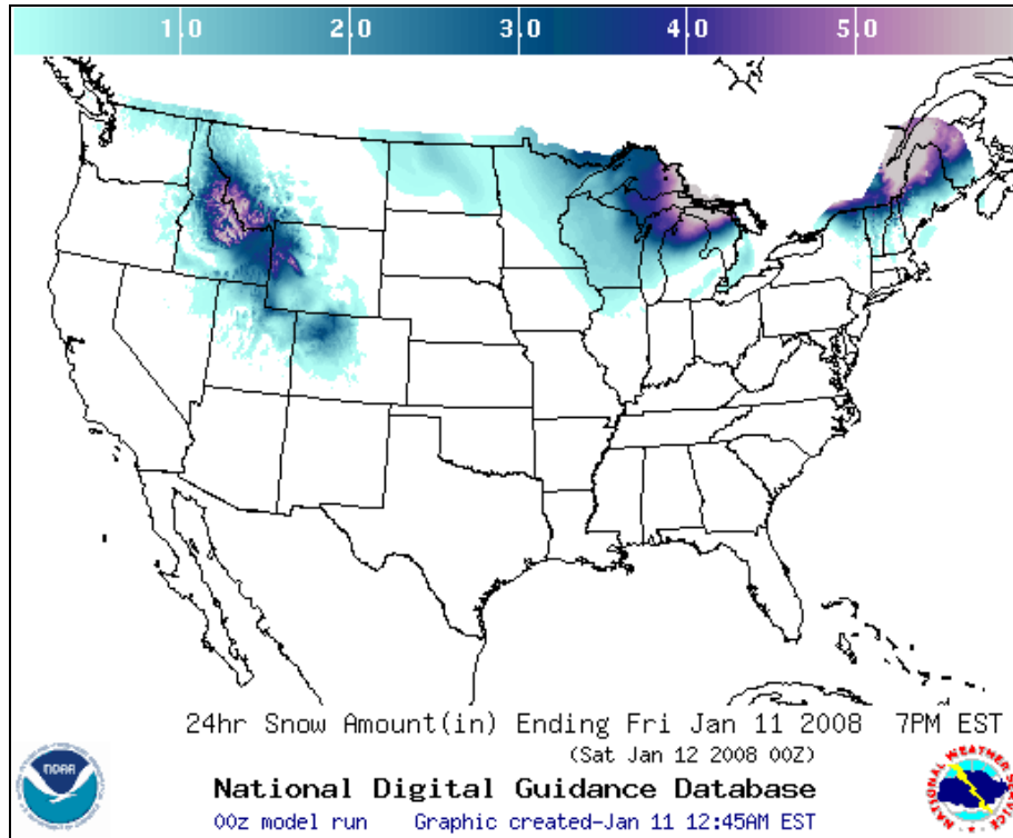
Figure 5. Gridded MOS 24-h snow fall amount ending Jan 12, 2008, 0000 UTC.
