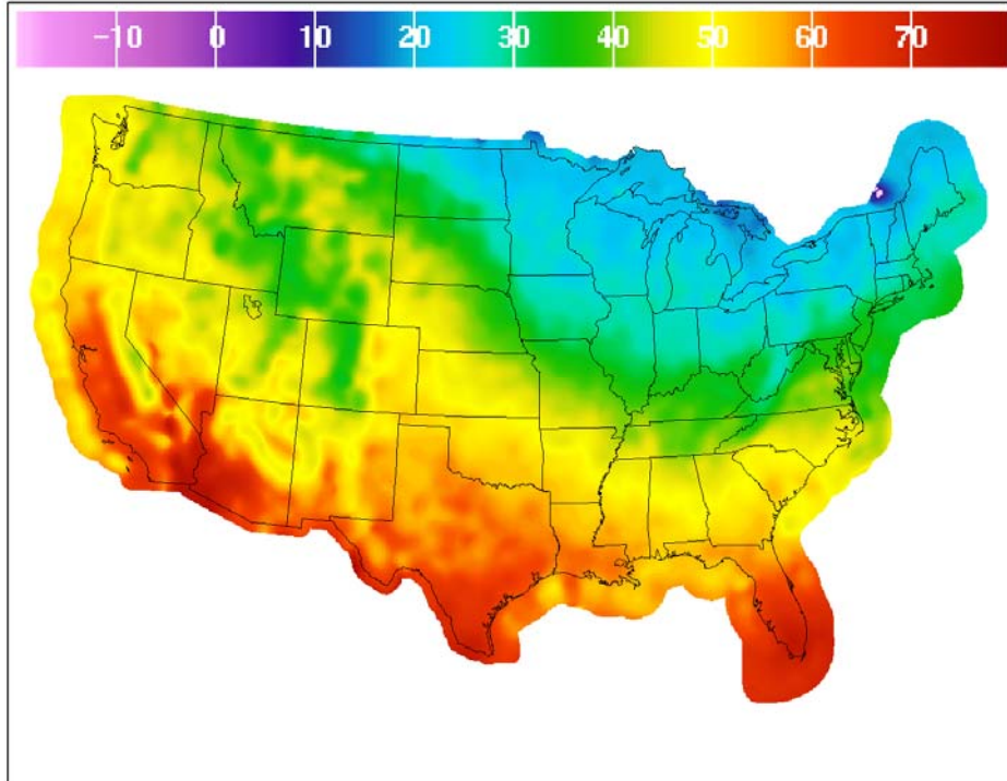
Figure 2. Analysis of the same data as for Fig. 1 except the land/water distinction and the VCE adjustment were not made.
