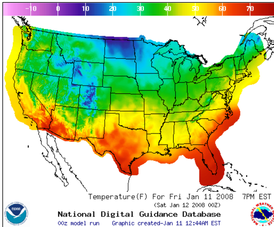
Figure 6. Gridded MOS Temperature °F at 0000 UTC on Jan 12, 2008
