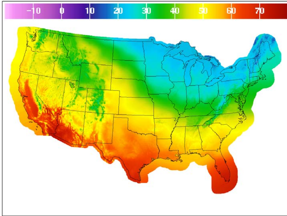
Figure 1. Analysis of 48-h temperature ( ^{\circ} F) MOS predictions based on June 26, 2007 data at 1200 UTC.
