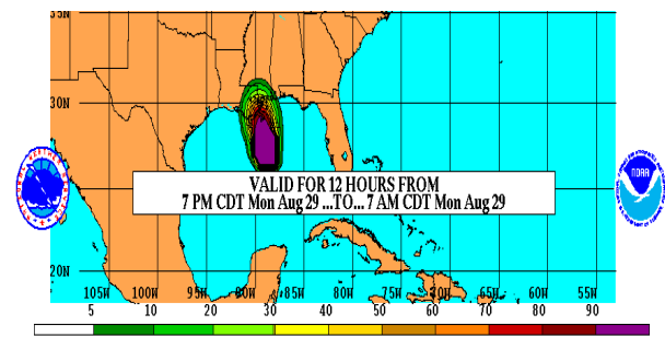
Figure 1. Experimental Tropical Cyclone Wind Probability, 64 kt wind, issued for the 12 h period ending at 7 AM CDT 29 August 2005.
