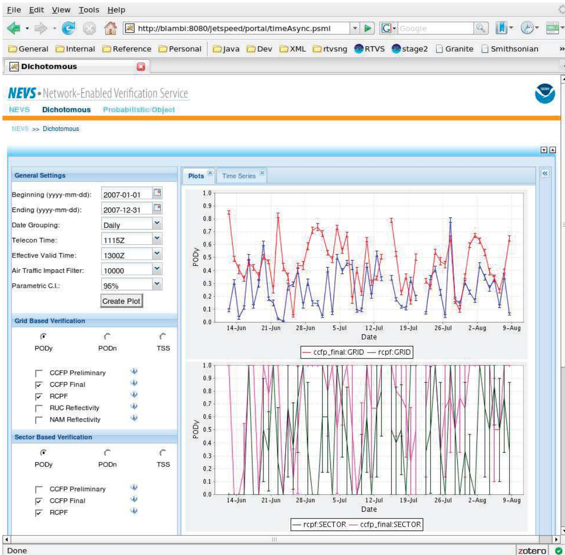
Figure 6. NEVS Use Case 1 - Extending traditional verification applications. Traditional verification features include sub-setting of data based on date and time, intercomparison of multiple products, selection among various statistics for comparison, and confidence intervals on statistics of interest. In addition, NEVS allows for easy extension of the traditional verification paradigm, incorporating the concept of air traffic planning periods and effective valid times, equalizing and comparing products based on user application not forecast production attributes, filtering the data by a user domain attribute, in this case a weather/traffic impact measure, and the introduction of the sector based dichotomous statistical approach (Matheson et al. 2008).
