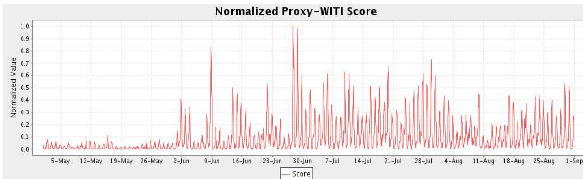
Figure 3. Normalized proxy WITI score per day from early May to mid Sept 2007 within the NAS.
