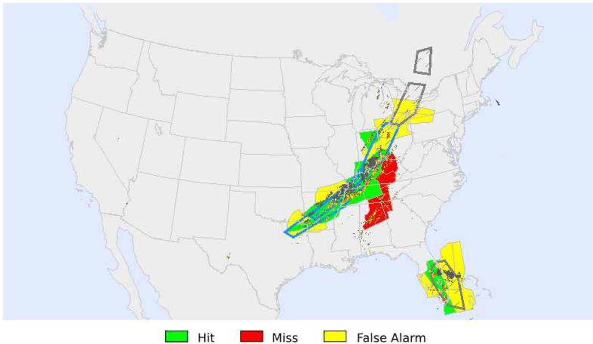
Figure 2. Sector-based verification of the 2-h CCFP Final forecast from 8 June 2007 issued at 1500 UTC. NCWD observations shown as well. Impacted sectors are color-coded to depict the verification results (from Kay et al. 2007).
