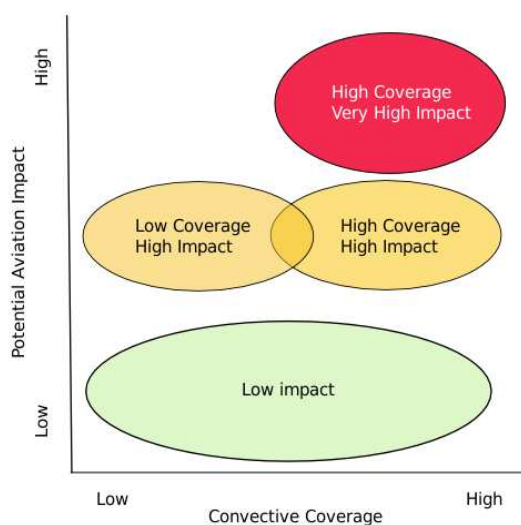
Figure 4. Schematic depiction of regimes that are of differing importance to aviation planning as a function of location of convection (as measured by potential aviation impact) and overall convective coverage over CONUS (Kay et al. 2007).
