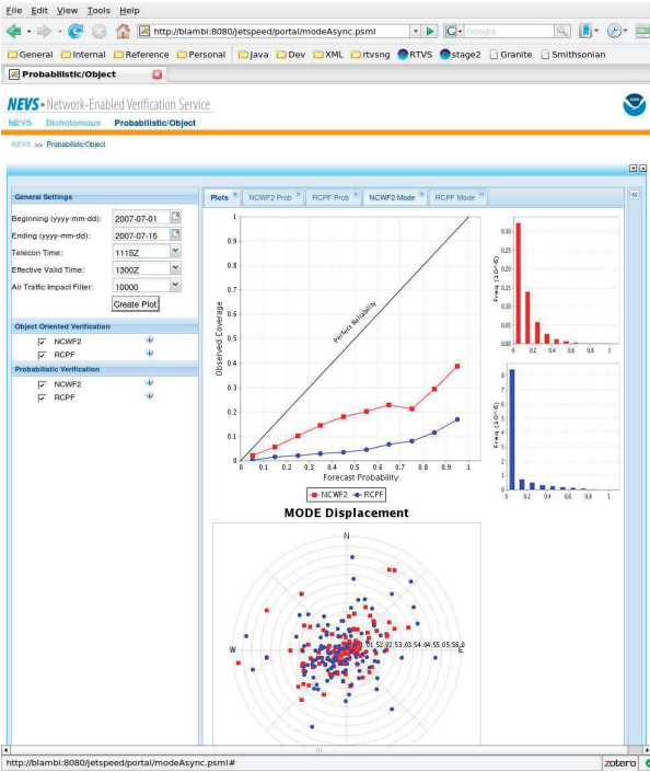
Figure 7. NEVS Use Case II - Facilitating new verification applications. The NEVS concept can also be utilized to build emerging verification applications. This graphic presents probabilistic and object oriented verification methods in a unified view that ensures the datasets: conform to the user viewpoint, are event equalized, are filtered along the same user-specific criteria (Matheson et al. 2008).
