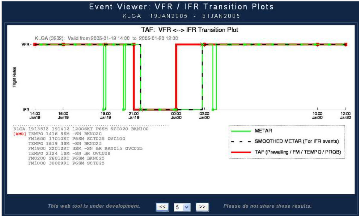
Figure 5. TAF lead-time metric event viewer. Green lines represent transition periods between observed IFR and VFR events. Red lines represent the transition periods as forecast by the TAF.
