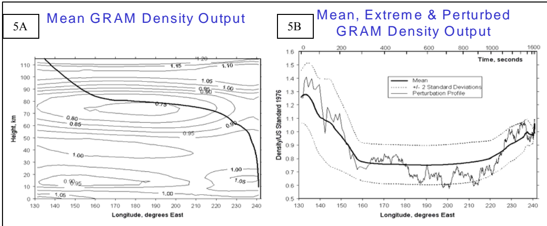
Figure 5. Resultant Earth GRAM-07 Mean and Extreme Density Values Computed Along the Example Mean January Trajectory. Figure 5A: Height vs. Longitude Cross Section of Density. Figure 5B: 2\sigma Density Envelopes, and One Monte-Carlo Density Perturbation Profile vs. Longitude. Density Expressed as a Ratio of US76 Standard Atmosphere Density.
