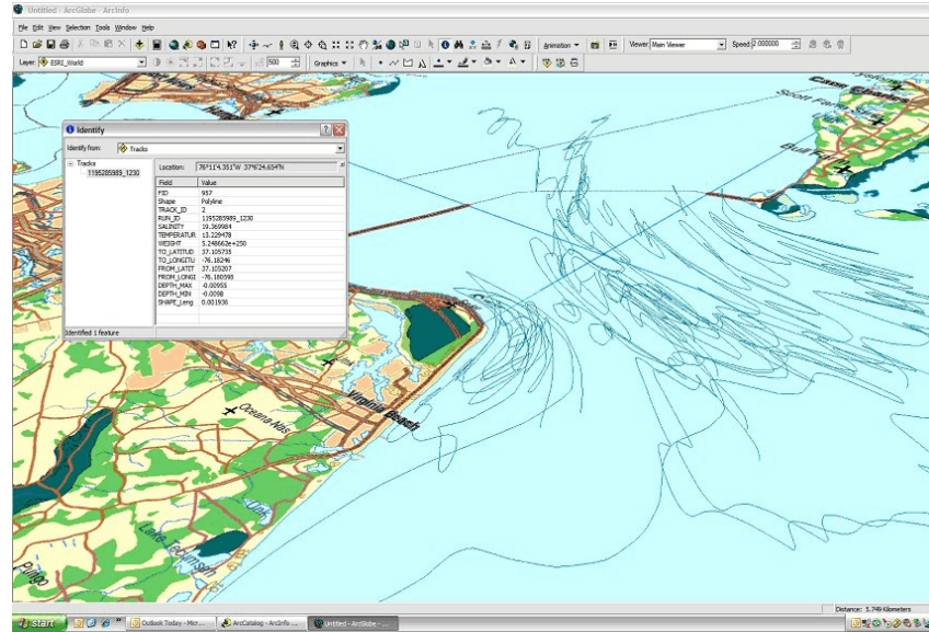
Figure 3 CBOLT output displayed in GeoFish GIS interface
