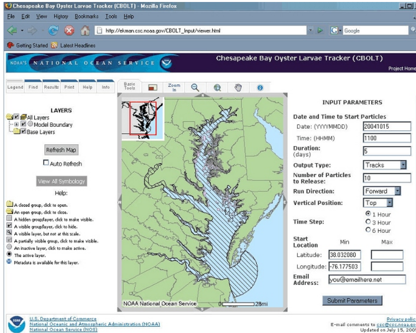
Figure 4 CBOLT/GeoFish interface
