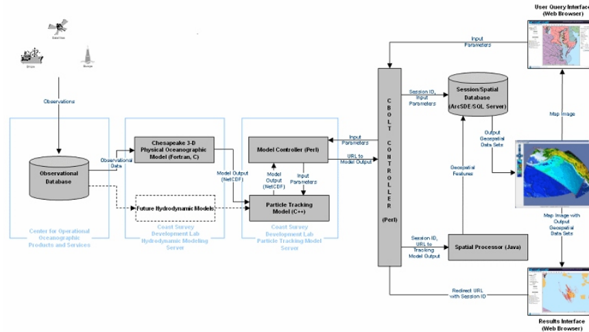
Figure 1 CBOLT/GeoFish architecture
