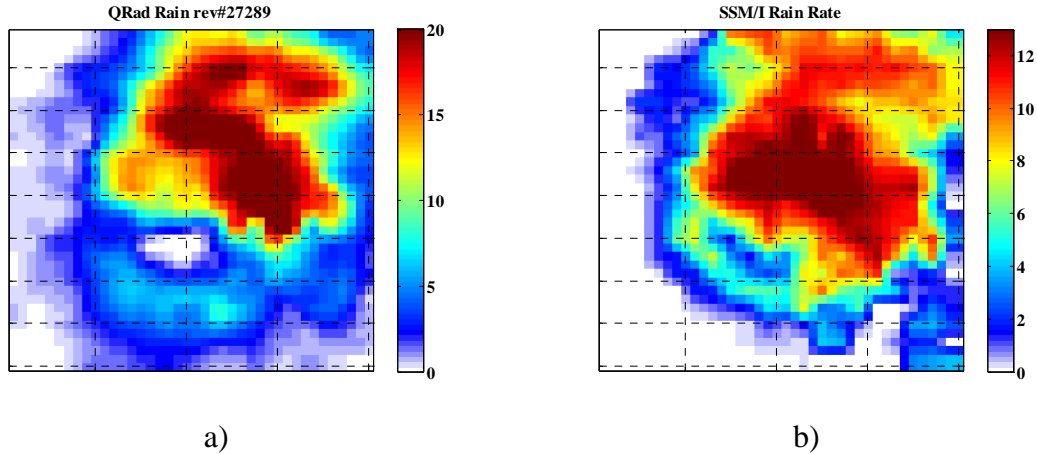
FIG. 1. Collocated rain comparisons for hurricane Ivan in 2004. a) QRad rain rate (rev#27289 at 23:59 UTC), b) SSM/I rain rate (at 23:44 UTC). Rain image x- and y-axis are relative longitude and latitude scales, with 12.5 km grid spacing.
