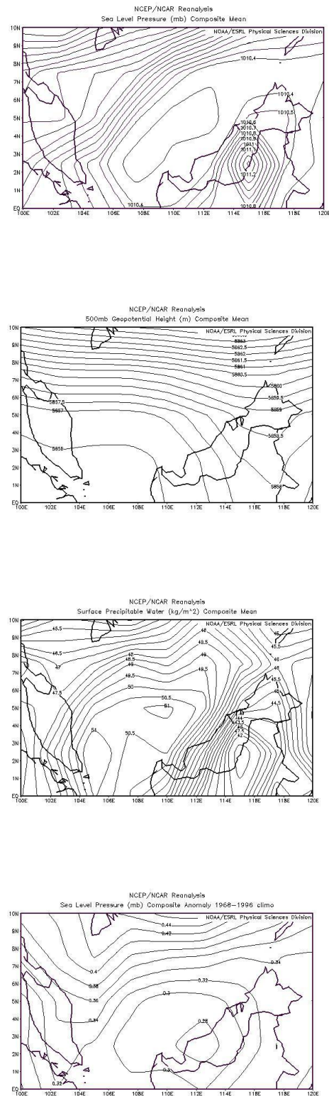
Figure 4. As in Fig. 2, except for the years in Table 7.
