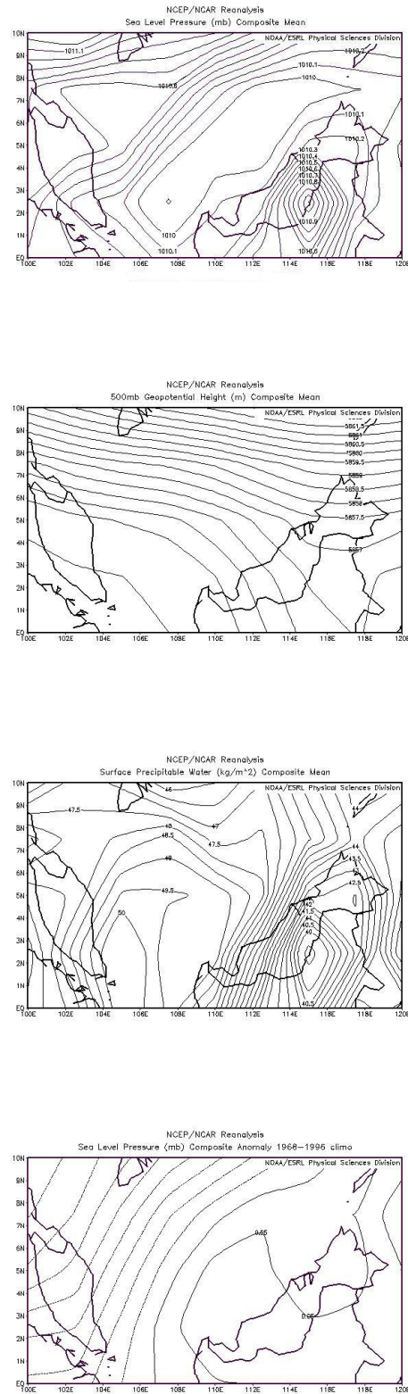
Figure 3. As in Fig. 2, except for the years in Table 6.
