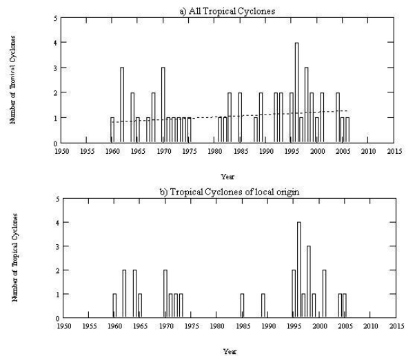
Figure 1. The time series of a) all tropical cyclones, and b) tropical cyclones of local origin occurring within the SCS region from 1960 – 2006. In a) the dashed line is the linear regression line.
