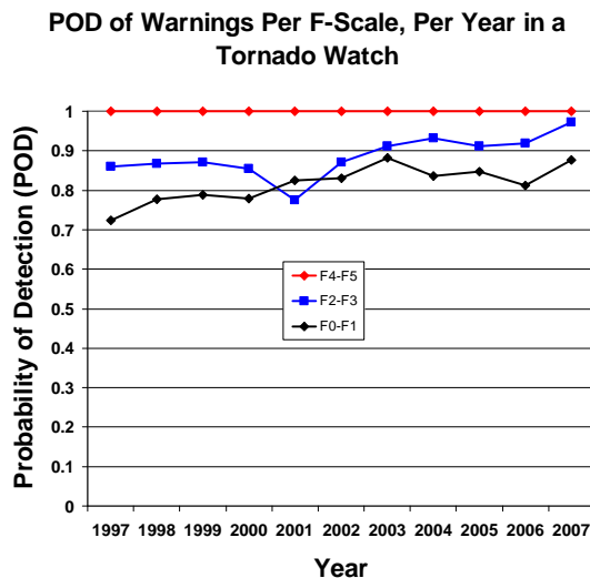
Figure 8: As in figure 3, except per F-Scale.
