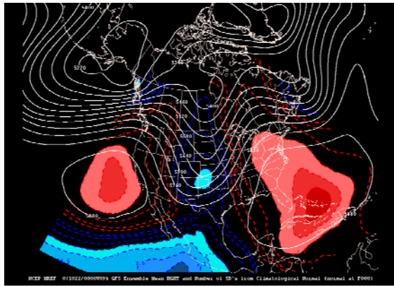
Figure 3. Date and time as in Fig. 1, except the ensemble mean height overlaid on the departure from normal (in units of standard deviation).
