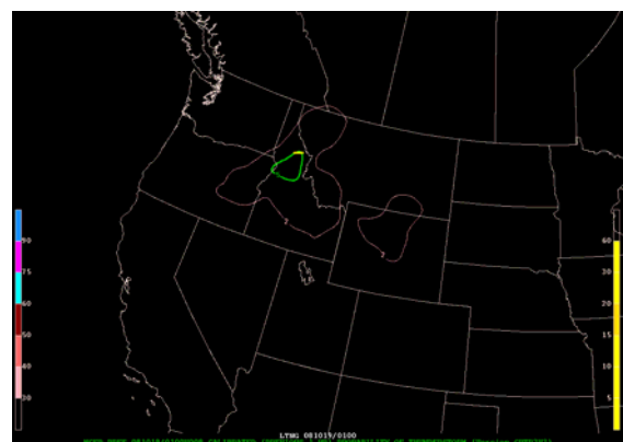
Figure 8. The 9 hour RREF calibrated probability of a thunderstorm valid 00 UTC to 01 UTC 19 Oct 2008. The CG lightning that occurred is indicated by the yellow symbol over northern Idaho.
