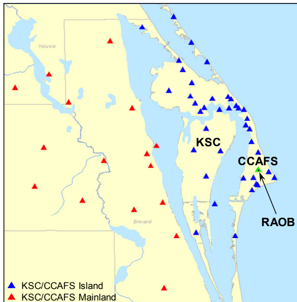
Figure 1. KSC/CCAFS wind tower network. Red triangles represent the mainland towers that may be eliminated. The XMR RAOB site is located at the green triangle.
