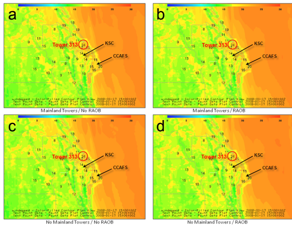
Figure 6. Comparison of the model forecast average winds (shaded) to the wind tower observations for the four scenarios of data withholding on 17 January 2008 at 1500 UTC. The wind tower observations show the 5 minute average wind speed and direction (wind barb) and peak speed (number at upper right of the wind barb). The model forecast peak wind speeds based on the (a) mainland towers and no RAOB , (b) mainland towers with the RAOB , (c) no mainland towers and no RAOB and (d) no mainland towers with RAOB . The model wind speed scale (kt) is shown at the top of each map. The location of the maximum peak wind speed is shown at Tower 313 by the red circle.
