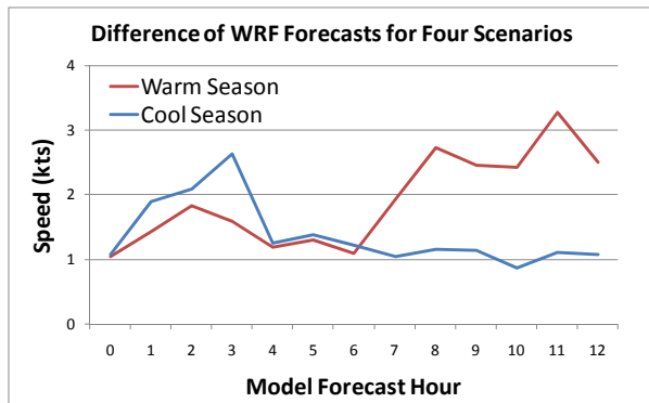
Figure 10. Chart showing the differences in WRF forecasts of maximum peak wind speed among the four scenarios for each hour of the model forecast for both the warm season (red line) and cool season (blue line).
