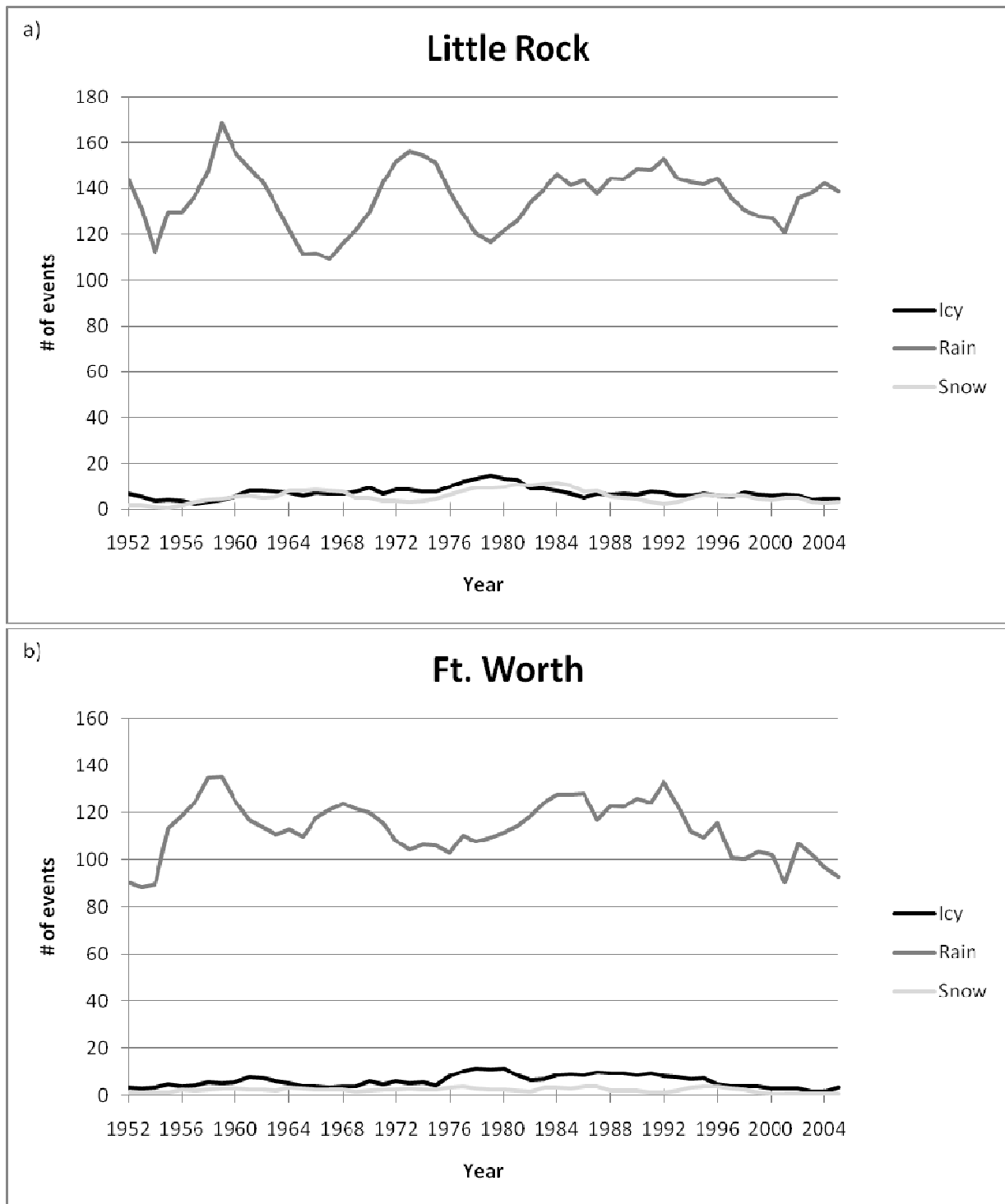
FIG 3. a,b. a) Shows the 5-year running mean (to factor out a lot of white noise) of the annual number of radiosonde indicated icy, rain, and snow events at Little Rock, AR. b) Same description as for a), for Ft. Worth, TX. Notice in both graphs the peak in icy days in the late 1970s.
