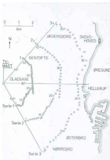
Figure 2: Tracer sampling-unit set up for the experiments in Copenhagen. Typically 20 locations in each arc situated in the actual plume direction for the individual experiments were used.
