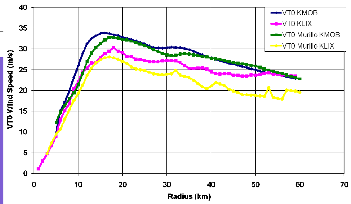
Tangential Wind Speed (Wavenumber 0) vs. Radius 1954Z 18 Jul 97
