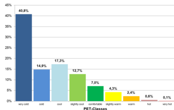
FIG. 1. PET-Classes at the urban climate station Freiburg for the period September, 1 st 1999 to December 31 st , 2009
