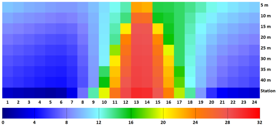
FIG. 3. Diurnal course of T_{mrt} (°C) for an urban canyon with Nord-South orientation, 15 m height and variable width (5 to 40 m) based on the data of the urban climate station and for the period September, 1st 1999 to December 31st, 2009
