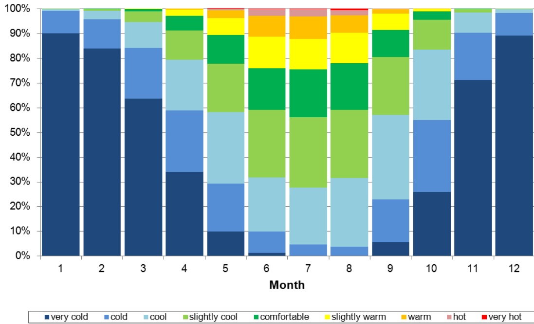
FIG. 2. Monthly Frequency distribution of PET at the urban climate station Freiburg for the period September, 1st 1999 to December 31st, 2009
