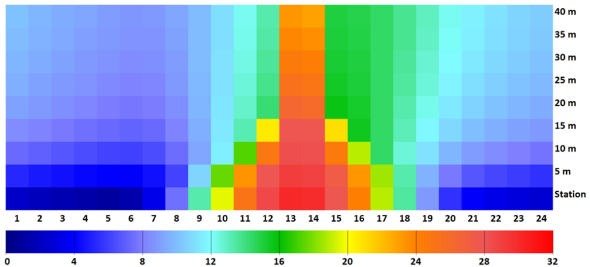
FIG. 5. Diurnal course of T_{mrt} ( ^{\circ}\text{C} ) for an urban canyon with North-South orientation, variable height (5 to 40 m) and 15 m width based on the data of the urban climate station and for the period September, 1st 1999 to December 31st, 2009
