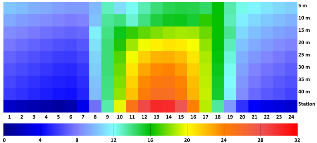
FIG. 4. Diurnal course of T_{mrt} ( ^{\circ}\text{C} ) for an urban canyon with East-West orientation, 15 m height and variable width (5 to 40 m) based on the data of the urban climate station and for the period September, 1st 1999 to December 31st, 2009
