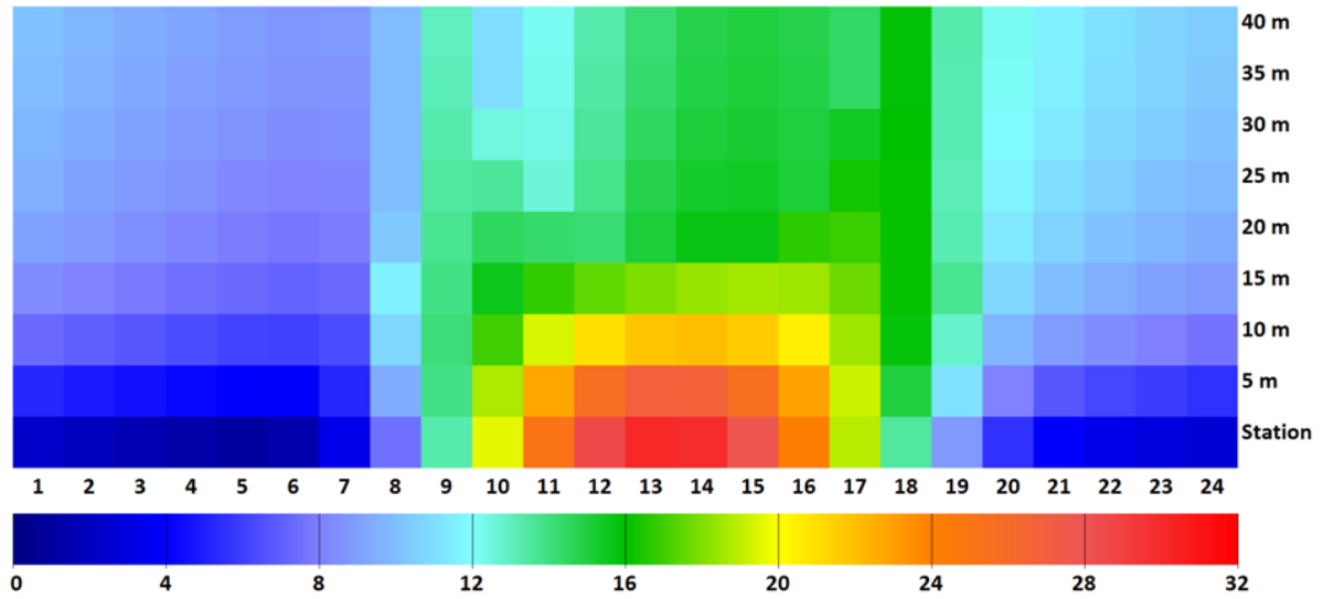
FIG. 6. Diurnal course of Tmrt (°C) for an urban canyon with East-West orientation, variable height (5 to 40 m) and 15 m width based on the data of the urban climate station and for the period September, 1st 1999 to December 31st, 2009
