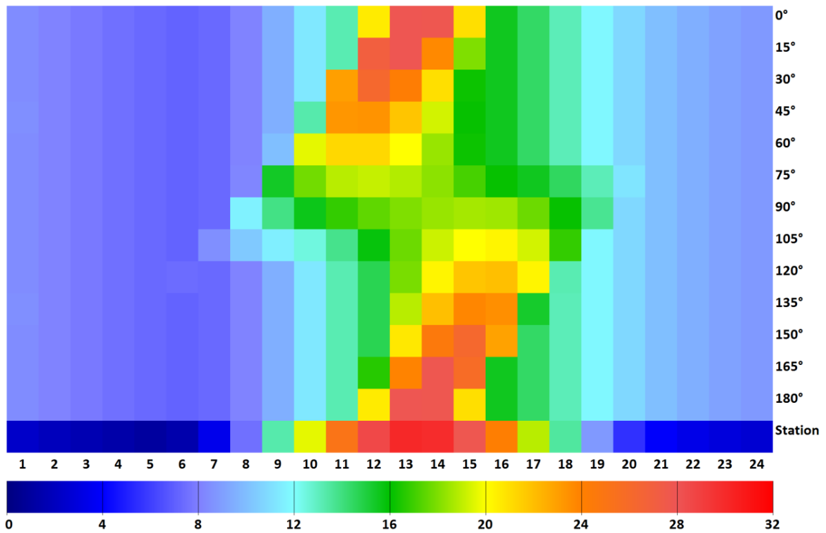
FIG. 7. Diurnal course of Tmrt (°C) for an urban canyon with steps of 15 ° rotation for a 15 m height and 15 m width based on the data of the urban climate station and for the period September, 1st 1999 to December 31st, 2009
