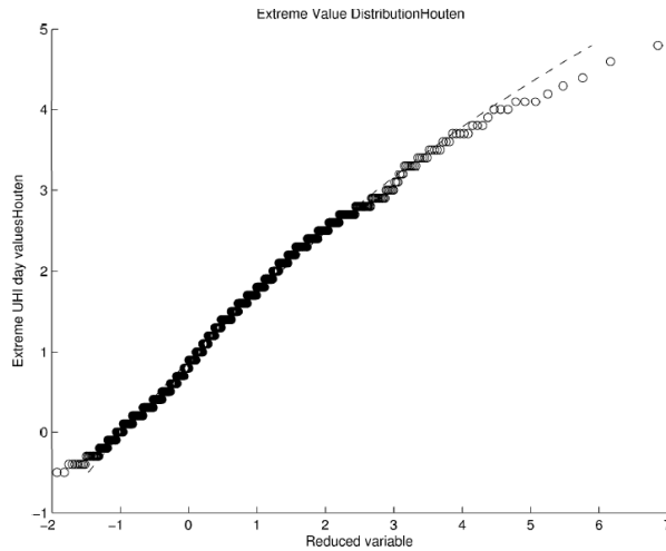
Fig. 5: Observed UHI_{max} versus the reduced variable, -\log(-\log(n/(n_{tot}+1))) , with n the n^{th} ranked observation and n_{tot} the total number of observations. Dashed line: fit to the GEV distribution.
