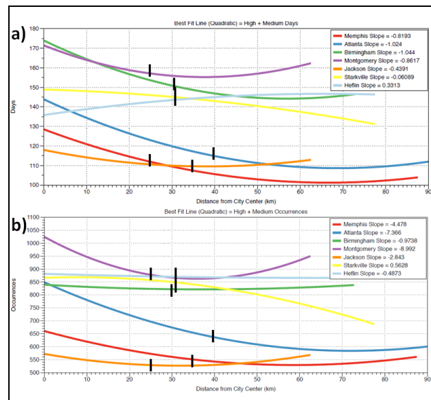
Figure 4. Quadratic line fits representing the relative frequency of a) total days \geq 40 dBZ and b) total number of 5-minute occurrences \geq 40 dBZ versus distance from city center for the seven domains examined. Various urban-rural buffers used (see Table 1) are represented by black line segments.
