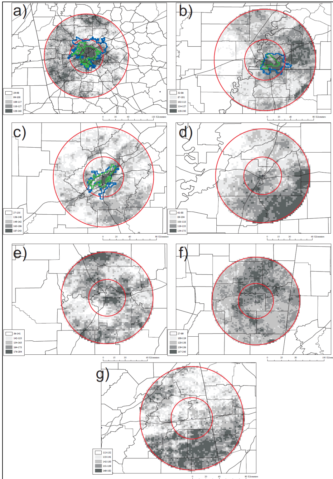
Figure 1. Frequency of June-August medium and high reflectivity days, or total days \geq 40 dBZ in each 2-km grid cell, for the 10-year period of record for a) Atlanta, b) Memphis, c) Birmingham, d) Jackson, e) Montgomery, f) Starkville control, and g) Heflin control. Red circles correspond to urban-rural buffers outlined in Table 1. For a-c, the blue (green) lines represent NLCD (USGS) urban delineations.
