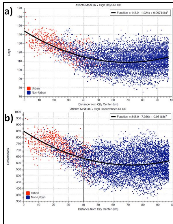
Figure 3. Quadratic line fits and associated scatterplots representing the frequency of a) total days \geq 40 dBZ and b) total number of 5-minute occurrences \geq 40 dBZ for each 2-km grid cell versus distance from city center in the Atlanta domain for the 10-year, June-August period of record. NLCD urban delineated cells are colored red, whereas non-urban cells are blue. The 40-km urban buffer for Atlanta is represented as solid line emanating from the x axis.
