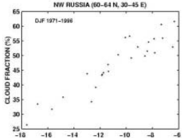
Figure 6: Scatterplot of low-level cloud fraction and surface air temperature in northwestern Russia (60-64N, 30-45E). Each point is December-February average over approximately 20 stations. The correlation is 0.93.
