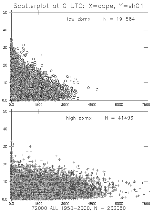
Fig. 2: Scatterplots of 00 UTC CAPE versus 0-1 km shear for all CONUS stations during the period 1950-2000, stratified by altitude of maximum parcel buoyancy "zbm x ". Panel (a) zbm x < 5.0 km above the surface; (b) zbm x > 7.5 km above the surface.
