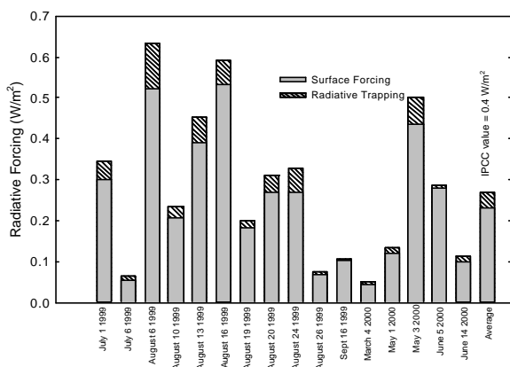
Figure 5: Summary of the surface forcing and radiative trapping of tropospheric ozone for the past two summers. The surface forcing fluxes are based on the FTIR measurements. The radiative trapping fluxes are based on simulations with the FASCOD3 model.
