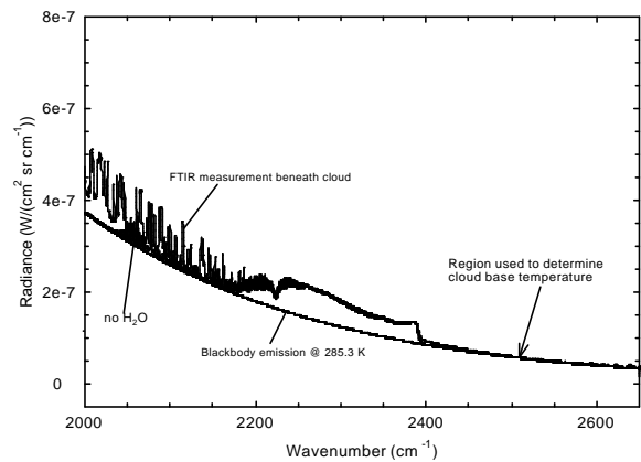
Figure 3: Use of the thermal emission spectrum to determine the cloud base temperature. Matching the emission intensity in the 2500 \text{cm}^{-1} region to an appropriate Planck blackbody emission curve yields the temperature of the cloud base.
