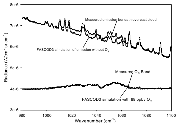
Figure 4: Determination of the ozone surface forcing beneath overcast cloud. A FASCOD3 simulation of the background emission in the absence of ozone was performed and subtracted from the measured total emission, which isolated the thermal emission band of tropospheric ozone. The radiative forcing was determined to be 0.43 \text{ W/m}^2 .
