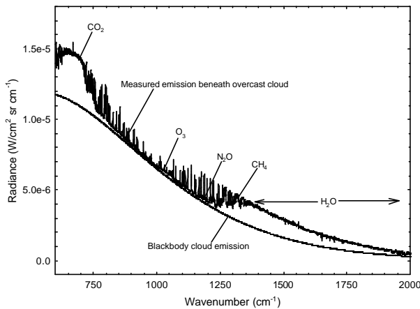
Figure 1: An example of the measurement of the thermal emission spectrum beneath overcast cloud. Several emission features are identified in the spectrum, including the large thermal contribution from the cloud itself, which behaves as a blackbody radiator.
