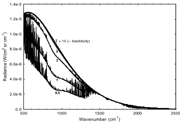
Figure 2: The thermal emission of clouds of varying optical depth, \tau . The spectra were simulated with the MODTRAN4 transmission model for varying cloud thickness. When an optical thickness of about eight is achieved then the cloud takes on the characteristic shape of a blackbody radiator. An optical depth of 8 translates to a cloud thickness of about 100m.
