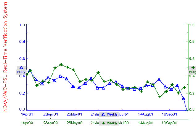
Figure 3. Time series of PODy for the 2-h CCFP forecast from 1 April – 30 September 2000 (+;) and 2001 ('triangle').
