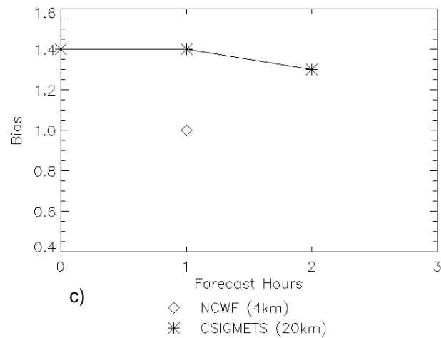
Figure 5 a-e. Verification statistics by forecast lead time for the 1-h NCWF (diamond); and the 0-, 1-, and 2-h C-SIGMETS ("*"; with speed and direction): (a) PODy; (b) FAR; (c) Bias; (d) % Area; and (e) CSI for the period from 1 April – 30 September 2001
