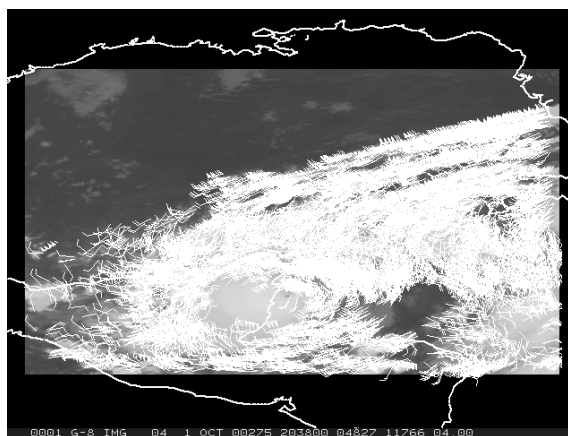
Fig. 1. Plot of GOES RS winds over the 100-400 hPa range during Hurricane Keith on 02 October 2000.
