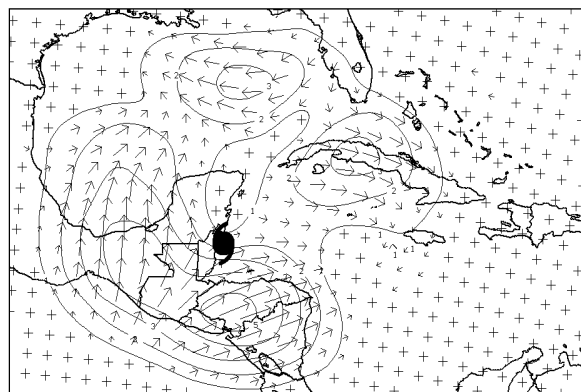
Fig. 2: 300 hPa wind differences between the experimental and control Eta analyses. The barbs show direction, while the isotachs show wind speed differences in \text{ms}^{-1}
