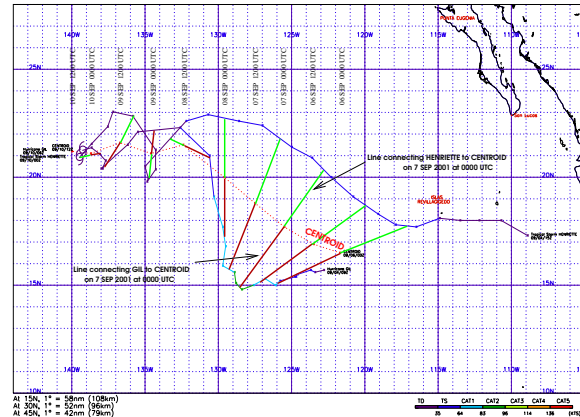
Figure 2: Tracks of Gil and Henriette, based on NHC advisories and GOES-10 imagery, shown with their centroid (dashed line). The thick lines connect the storm tracks to the centroid (dark is G-C, light is H-C) at nine times. Before merging, the storms had rotated approximately 540^\circ about the centroid.
