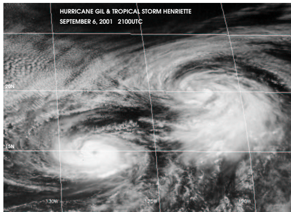
Figure 1: Hurricane Gil and Tropical Storm Henriette at 2100 UTC on 6 September 2001. Henriette is to the northeast. Longitude and latitude lines are 5 degrees apart, and Gil is at 15N 128W.
