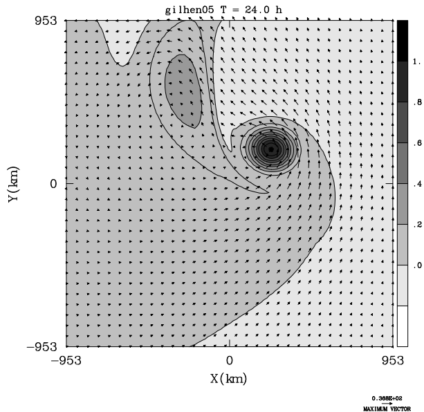
Figure 4: Isolines of normalized relative vorticity and horizontal wind at t = 24 h for a VICBAR simulation initialized with Gil and Henriette idealized as two circular vortices.
