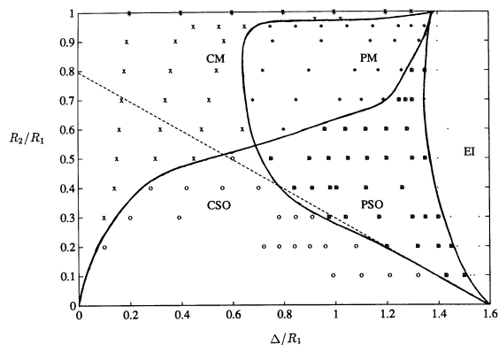
Figure 3: Flow regimes for CD/CS calculations of the inelastic interactions of unequal Rankine vortices. Five regimes are found, depending on the size ratio R_2/R_1 and the dimensionless gap \Delta/R_1 (from Dritschel and Waugh 1992).
