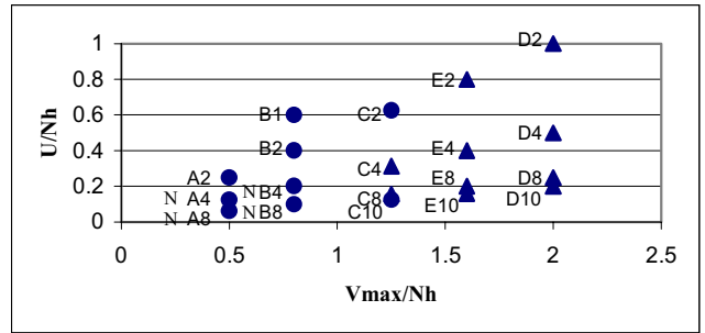
Fig. 1: Continuous (in triangles) or discontinuous (in circles) track of circulation centers for cases (see Table 1) performed. Tracks with northward deflection are denoted by N, otherwise they are deflected toward south.
