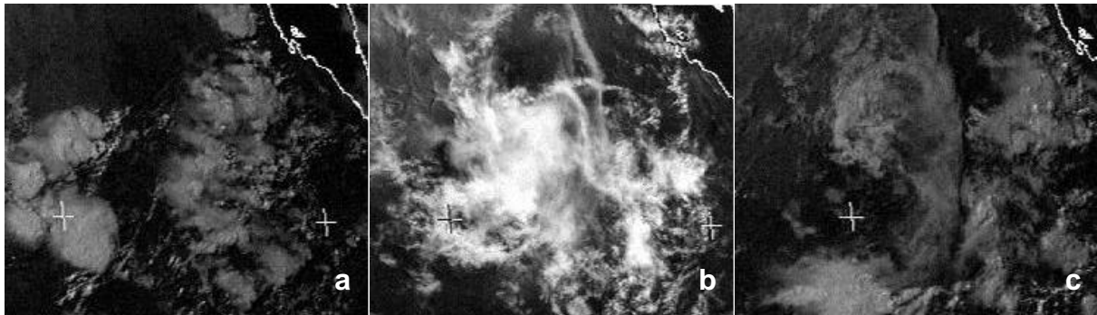
Figure 1. METEOSAT-7 VIS images for a) 1430 UTC 28 July 2000, b) 0830 UTC 29 July 2000, and c) 1430 UTC 29 July 2000. Leftmost cross-hair denotes 10°N, 30°E. Images from University of Nottingham, UK.
