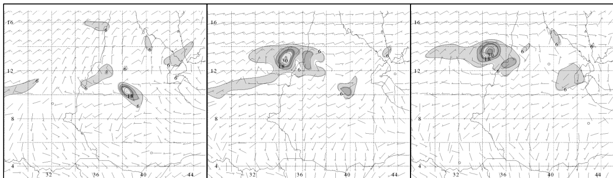
Figure 2. MASS-simulated relative vorticity and wind vectors at 660 mb corresponding to a) 1800 UTC 28 July 2000, b) 0600 UTC 29 July 2000, and c) 1200 UTC 29 July 2000. Vorticity contoured and shaded every 6 \times 10^{-5} \text{ s}^{-1} . Wind vectors in units of \text{ms}^{-1} .
