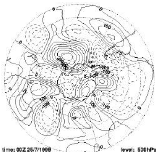
Figure 1: Anomaly of geopotential height at 500hpa for 00Z 25 July 1999. The contour interval is 50m and negative contours are dashed.
