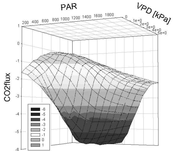
Figure 2: \text{CO}_2 -Flux as a function of PAR and Vapor Pressure Deficit (VPD) for all 1998 data, when VPD reached large values due to 78 day drought. \text{CO}_2 -Flux drops off rapidly with VPD.
