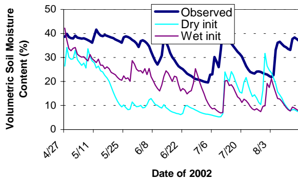
Figure 2. Forecast improvement by correcting initial soil water content using the observations. The forecast started on 27 April, 2002.
