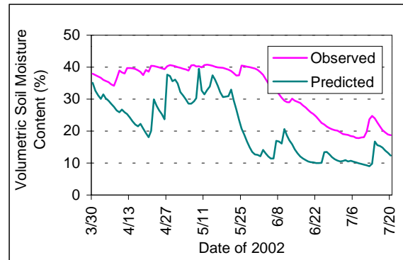
Figure 4. Validation of soil moisture forecast at Spickard, MO. The forecast started on 30 March, 2002.
