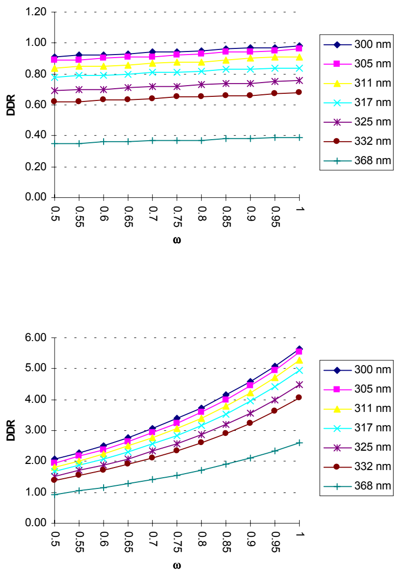
Figure 3. (a) Sensitivity of diffuse-to-direct ratio (DDR) to single scattering albedo ( \omega ) in TUV4.1 at AOD=0.05. (b) same as (a) at AOD=1.00.
