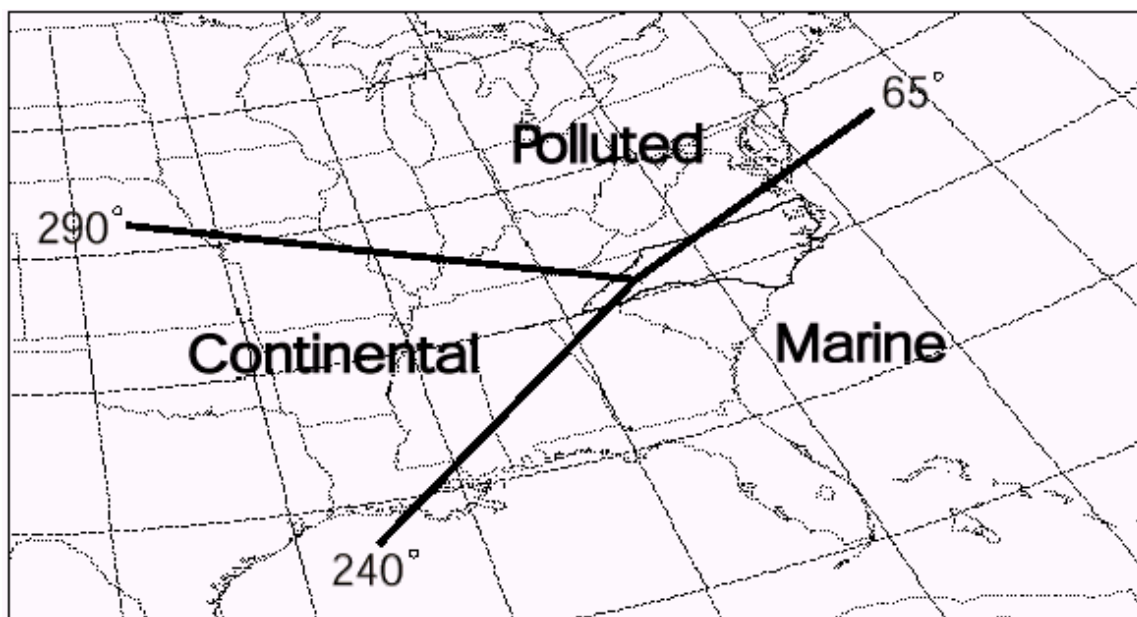
Figure 2. Map of the United States illustrating the geographical location and classification of the different air mass types influencing the research site in Black Mountain, NC.
