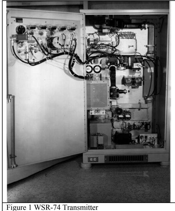
Figure 1 WSR-74 Transmitter
