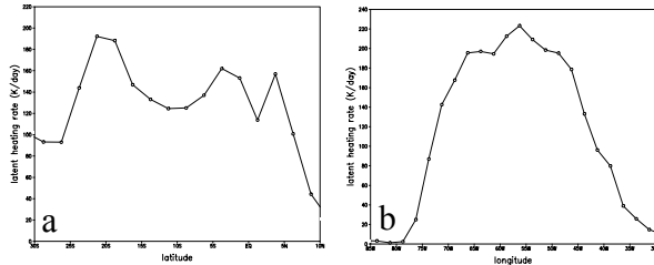
Figure 2. North-south in 45° W and (b) East-west in 15° S (b) distribution of latent heating rate, that represents the atmosphere heating by condensation of water vapor.
