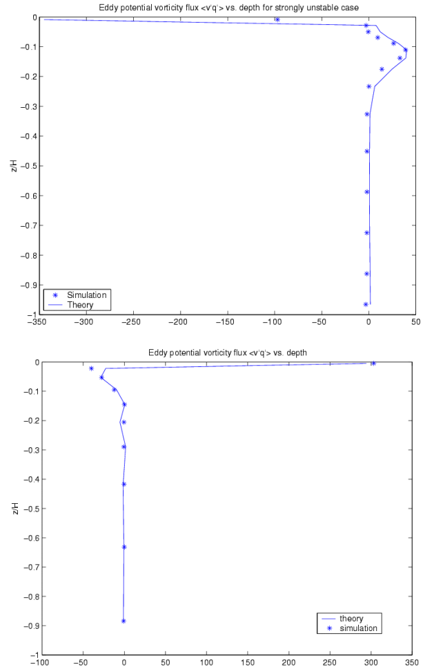
Figure 1: Top: profile of northward eddy potential vorticity flux \overline{v'q'} from 256^2 by 15-layer simulation (asterisks) using mean profiles that are interpolations from the shear and potential density profiles generated by a primitive equation simulation of the North Atlantic, compared to theory based on (17) with (20) and (21) (solid). Bottom: profile of northward eddy potential vorticity flux \overline{v'q'} from 512^2 by 10-layer simulation (asterisks) using mean profiles taken from NATRE, compared to same theory (solid).
