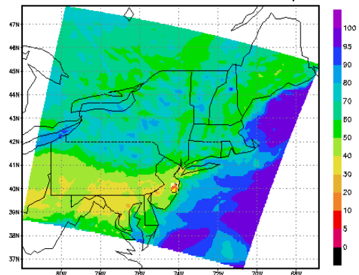
Surface RH in % valid at 1700UTC on JUN 02, 2002
