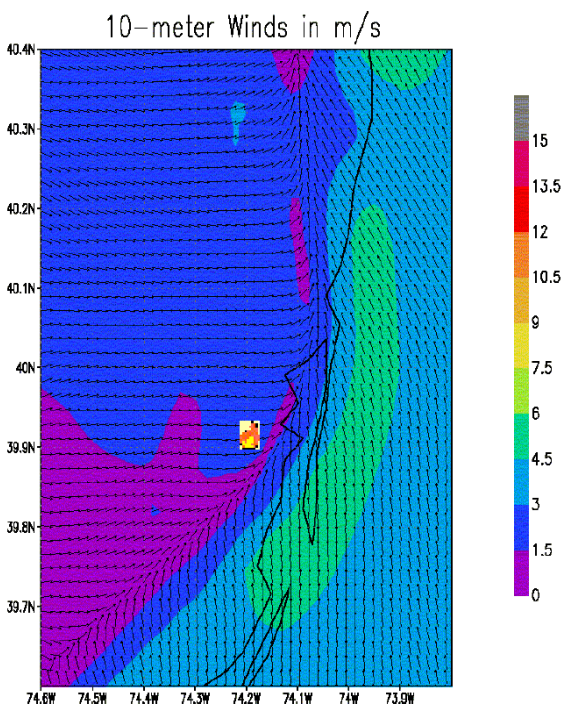
Figure 3: Simulated surface wind valid at 2300UTC June 3, 2002. The location of the fire is indicated by an orange flame icon.
