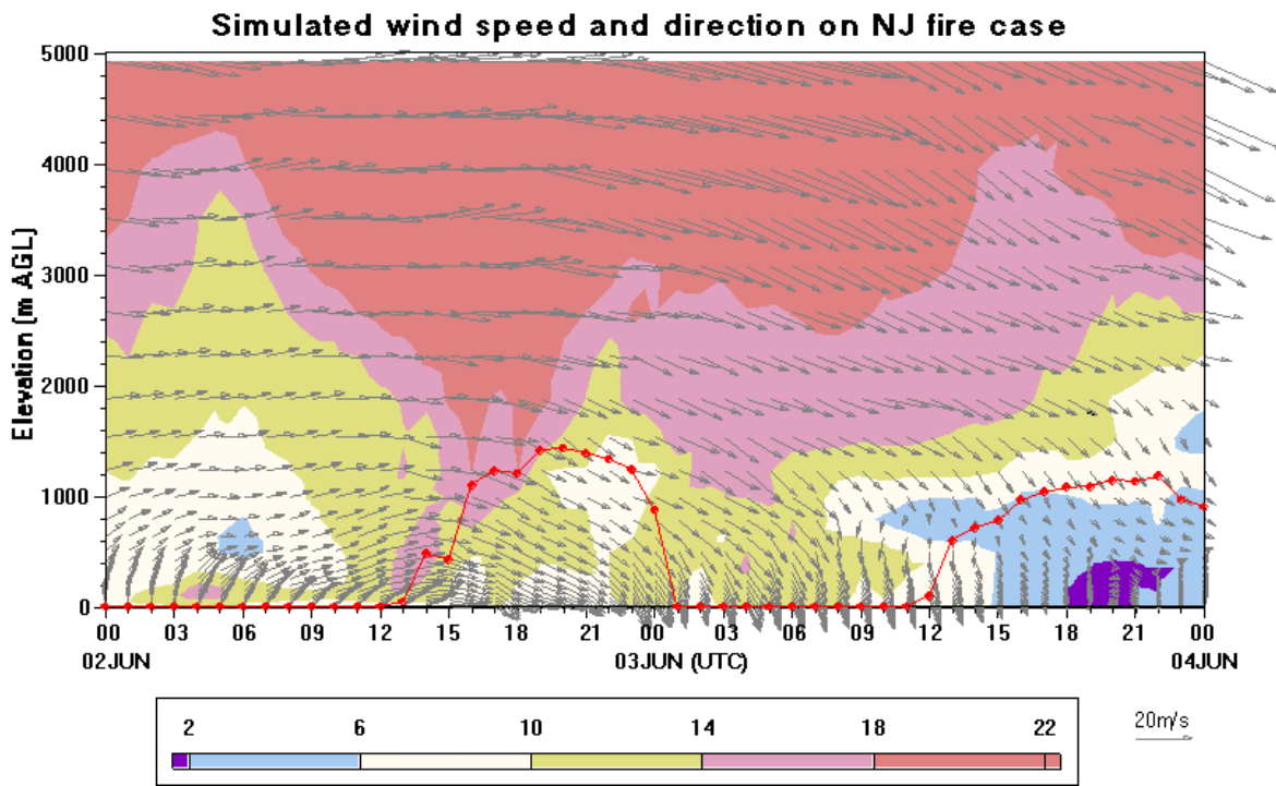
Figure 5: Time-height cross section of simulated wind speed (in m/s), horizontal (x-y plane) direction (vector arrows), and mixed-layer height (red line) valid from 0000UTC June 2, 2002 through 0000UTC June 4, 2002.
