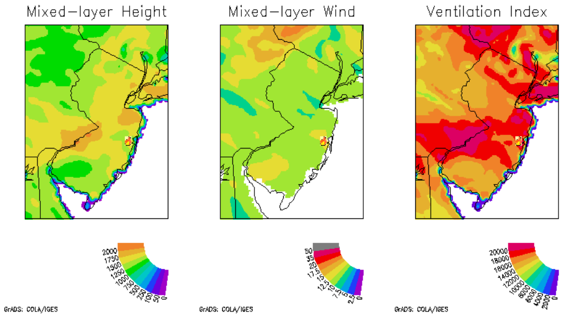
Figure 4: Three-panel plot of simulated mixed-layer height (in meters), mixed-layer-average wind speed (in m/s), and ventilation index (in m 2 /s 2 ) valid for 2000UTC June 2, 2002.
