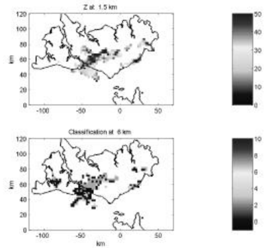
Fig. 2 Example of reflectivity and microphysical classification. Note that 9 corresponds to wet graupel here to highlight mixed phase areas.
