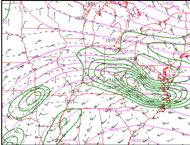
Figure 6. Eta analysis at 00 UTC 16 February 2003. 850-700 hPa thickness (m) pink lines, layer mean wind (kts) in barbs, 850 hPa frontogenesis ( K 100 km^{-1} 3 hr^{-1} ) in green, and MSLP (hPa) dashed lines.
