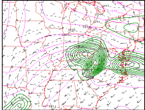
Figure 7. Same as Fig. 6 except Eta 12-hour forecast valid at 12 UTC 16 February 2003.
