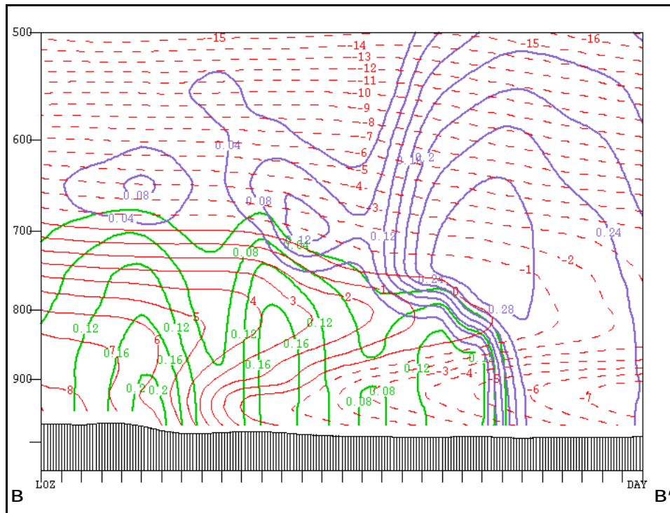
Figure 9. Vertical cross-section taken along the black line (B-B') in Fig. 8, with data interpolated to
