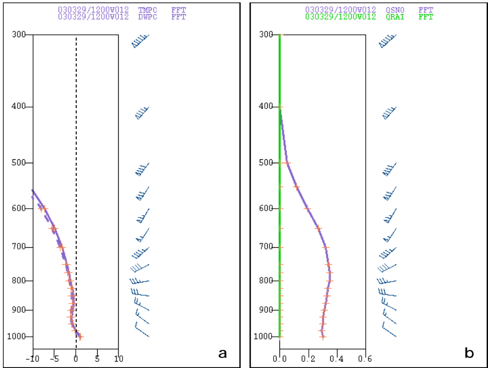
Figure 12. Point sounding at Frankfort, KY (FFT) of the MM5 data at the same time as in Fig. 11. The left-hand plot (a) is a log-p plot of temperature (solid) and dew point (dashed). The right-hand chart (b) is a log-p plot of the snow (purple) and rain (green) hydrometeor mixing ratios ( g\ kg^{-1} ). The approximate location of FFT is noted in Fig. 11 by the blue star.
