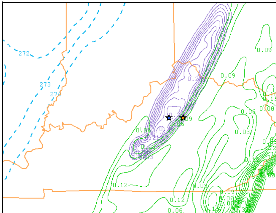
Figure 11. Experimental precipitation type chart valid at 12 UTC 29 March 2003, a 12 hour forecast from the 00 UTC 29 March MM5 initialization. Contours are the same as in Fig. 4. All ground temperatures to the right of the 274 K line are at or above 274 K. The approximate location of Frankfort is shown by the blue star and Lexington by the orange star.
