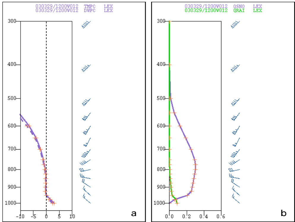
Figure 13. Same as Fig. 12, except at Lexington, KY (LEX). The approximate location of LEX is noted in Fig. 11 by the orange star.
