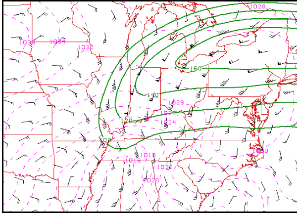
Figure 3. 00 UTC 05 December 2002. 250 hPa isotachs (kts) in green, 250 hPa ageostrophic wind component barbs (kts), and MSLP (hPa) in dashed pink.
