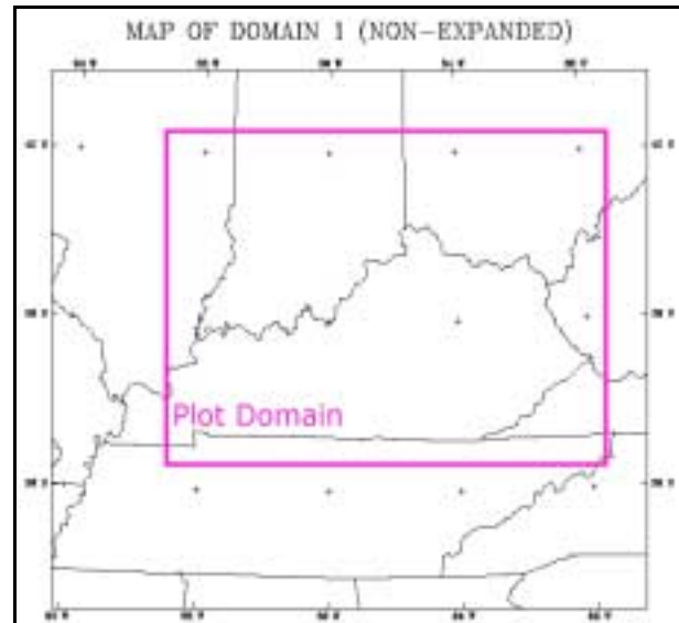
Figure 2. The LMK-MM5 grid domain (outer rectangle) and precipitation type plot boundary (inner rectangle).
