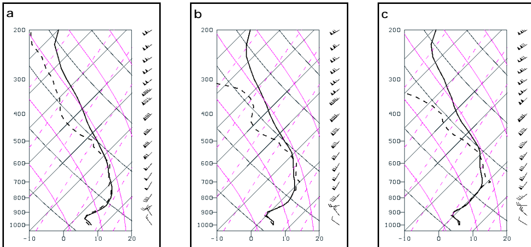
Figure 10. Sample point soundings (skew-t) taken within axis of 700 hPa upward vertical motion associated with 700 hPa frontogenesis maximum. Eta initialized at 00 UTC 29 March 2003: (a) 3 hour forecast, (b) 6 hour forecast, and (c) 9 hour forecast. Temperature ( ^{\circ}\text{C} ) is shown with solid lines, dew point in dashed lines, and wind (kts) in barbs. Advections were taken into account within the south-southwesterly flow above a cold frontal interface to determine the locations of each sounding. This gives one a "crude" Lagrangian view. Note the supersaturation in the soundings, occasionally seen in Eta output during strong vertical motion events.
