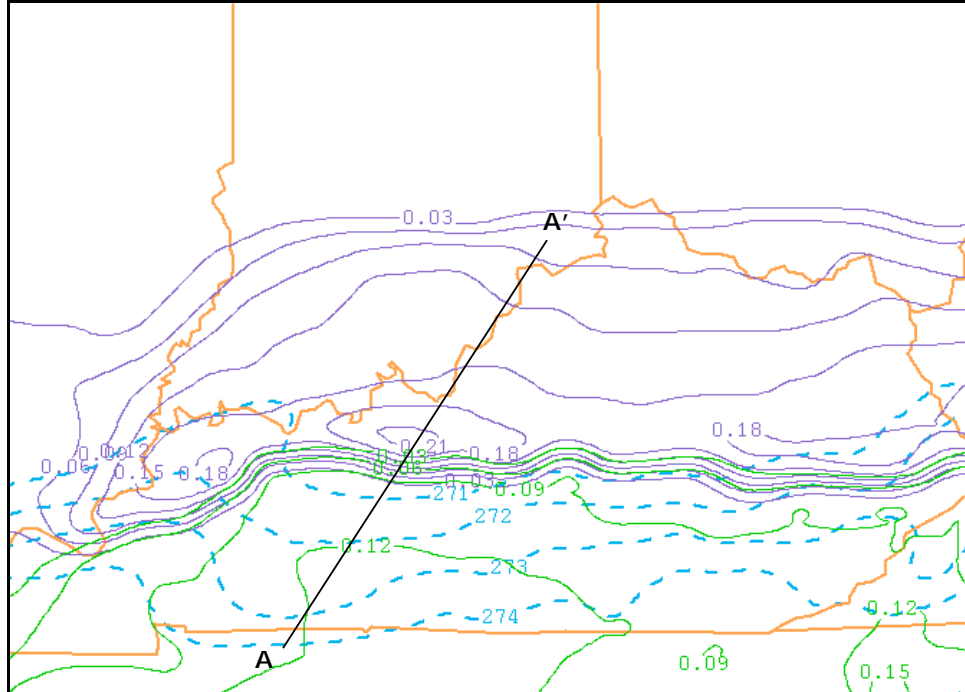
Figure 4. Standard LMK-MM5 experimental precipitation type chart. Snow (purple) and rain (green) hydrometeor mixing ratios ( \text{g kg}^{-1} ) on the 0.995 sigma surface, and ground temperatures in the top few cm of the model soil in blue dashed lines (K). Only “critical” temperatures around 273 K are noted. This particular chart is valid at 00 UTC on 5 December 2002, a 24 hour forecast from the MM5 initialization at 00 UTC on 4 December. The black line (A-A’) refers to the vertical cross-section in Fig. 5.
