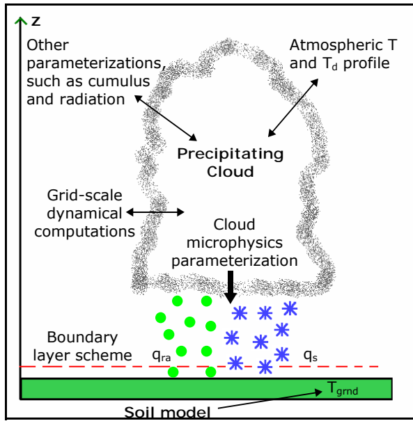
Figure 1. Schematic diagram as described in text.
