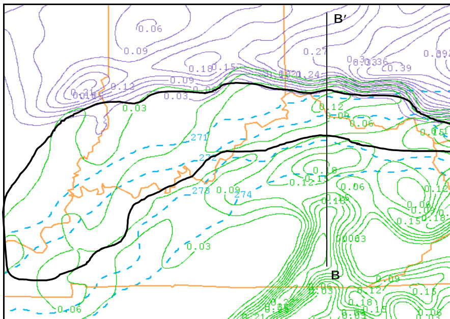
Figure 8. Experimental precipitation type chart valid at 12 UTC 16 February 2003, a 12-hour forecast from the 00 UTC 16 February MM5 initialization. Contours are the same as in Fig. 4. The general area of forecast "freezing rain" is highlighted with the freehand black line. The black line (B-B') represents the vertical cross-section in Fig. 9.
