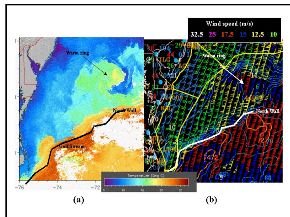
Fig. 2. SST AVHRR 3 day composite (a) and 25 km QuikSCAT winds (b). In (b) wind speeds are colored as indicated in the table in the upper right hand corner. The location of the North Wall of the Gulf Stream is shown by a dark line in (a) and white line in (b). Contours in (b) are SST in degrees F from the NESDIS 14 km resolution SST analysis.
