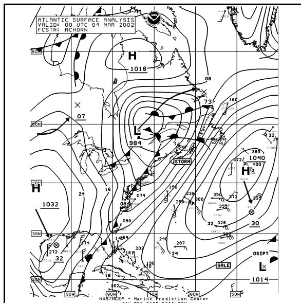
Fig. 1. OPC operational surface analysis for the western North Atlantic from 0000 UTC 4 March 2002.
