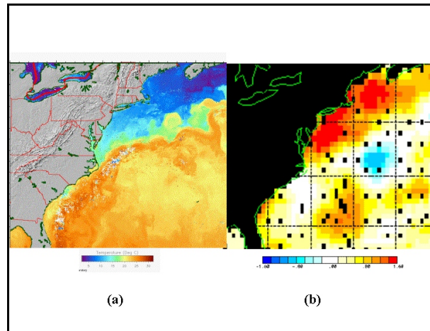
Fig. 5. Seven day AVHRR SST composite from April 15, 2002 in (a). Bias of 10 m winds from the NOAA Western North Atlantic Wavewatch III Wave Model as compared to altimeter derived winds (b).
