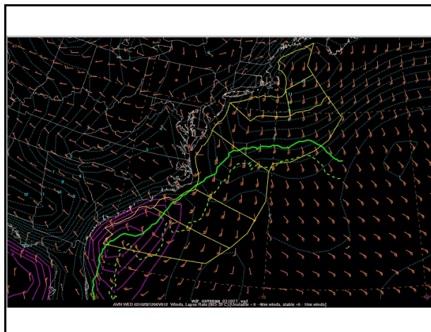
Fig. 7. GFS based surface to 925 hPa lifted index with magenta contours negative indicating instability. Cyan dashed contours are positive and indicate areas of stability. Plotted winds are a mix of 40 m high winds in unstable areas and 10 m winds in stable areas. The Navy OFA Gulf Stream analysis is shown as in Fig. 6.
