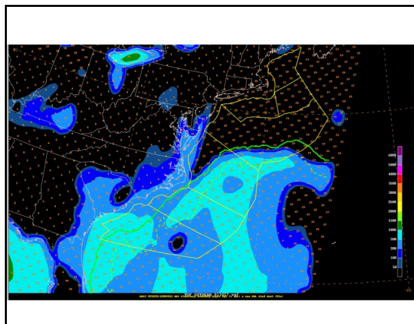
Fig. 8. NCEP RUC model height of the MABL (colored contours) and maximum MABL wind gust (numeric values) in knots for 1200 UTC 29 Oct 2003.
