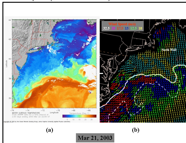
Fig. 4. 3-day SST composite from AVHRR (a) and QuikSCAT winds from March 21, 2003 (b). The U.S. Navy OFA Gulf Stream North Wall (white solid line) and South Wall (white dashed line) analyses are shown in (b).
