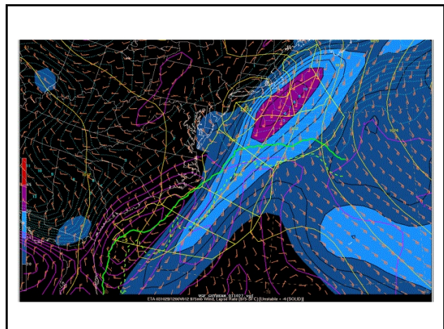
Fig. 6. Eta model forecast from 29 Oct 2003 of 975 hPa-surface lifted index as purple solid lines where negative and cyan dashed lines where positive. Contours are 975 hPa isotachs. Yellow lines are surface isobars at a 4 hPa spacing. Wind barbs are 975 hPa winds. The green solid line is the north wall of the Gulf Stream from the U.S. Navy OFA analysis.
