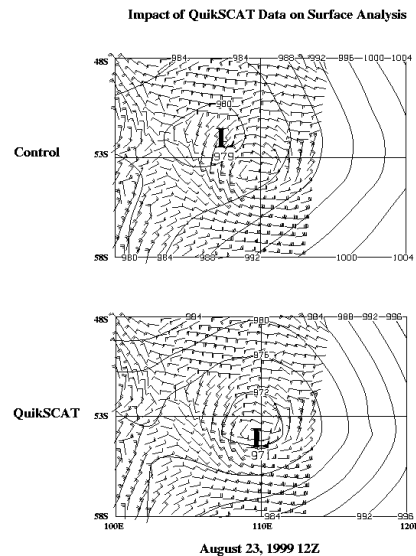
Fig. 5. Top: Control Sea Level Pressure analysis, which does not conform to the QuikScat wind data. Bottom: Sea Level Pressure analysis using QuikScat data., showing a much improved agreement.
