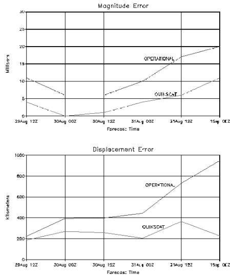
Fig. 8. Magnitude and displacement errors of Hurricane Cindy in the NCEP system over a 60 hour period.
