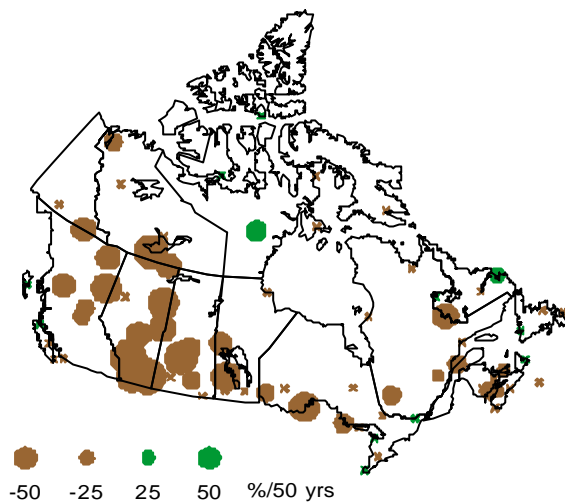
Fig. 5: Trend in Percentage Winter Precipitation Change during 1954-2003 relative to 1961-90. Green (brown) dots represent increasing (decreasing) precipitation statistically significant at the 5% level. Crosses represent insignificant trends.
