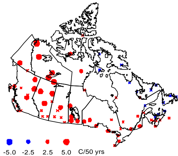
Fig. 4: Trend in Winter Temperature during 1954-2003. Blue (red) dots represent decreasing (increasing) temperature statistically significant at the 5% level. Crosses represent insignificant trends.
