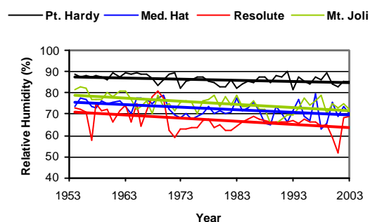
Fig. 1: Trend in Winter Relative Humidity for 4 Stations Located in Different Climate Zones. 1) Port Hardy, British Columbia, 2) Medicine Hat, Alberta 3) Resolute, Nunavut 4) Mont Joli, Quebec.
