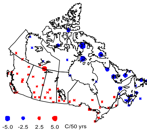
Fig. 3: Trend in Winter Dew Point Temperature during 1954-2003. Blue (red) dots represent decreasing (increasing) dew point statistically significant at the 5% level. Crosses represent insignificant trends.
