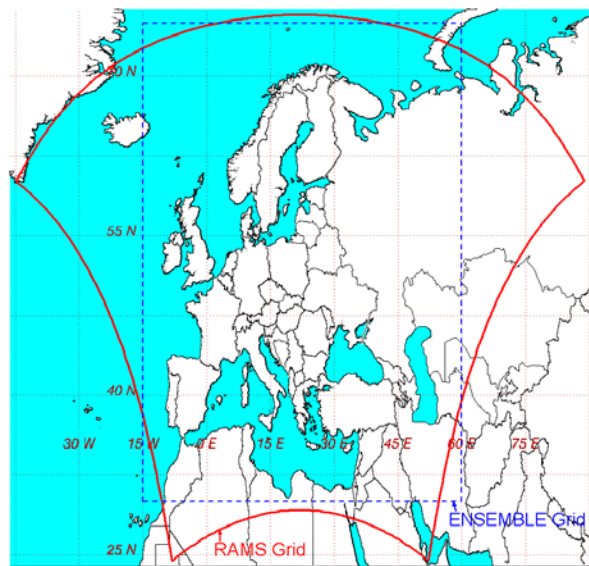
Figure 1: ENSEMBLE domain and SRTC RAMS grid.
