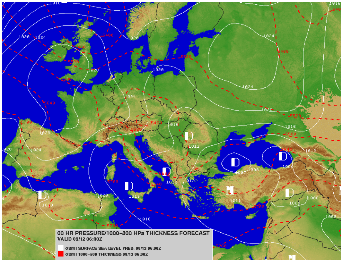
Figure 8-5 GSM Analysis of Surface Pressure and 1000-500 hPa Thickness, valid at Sept 12, 06 UTC
