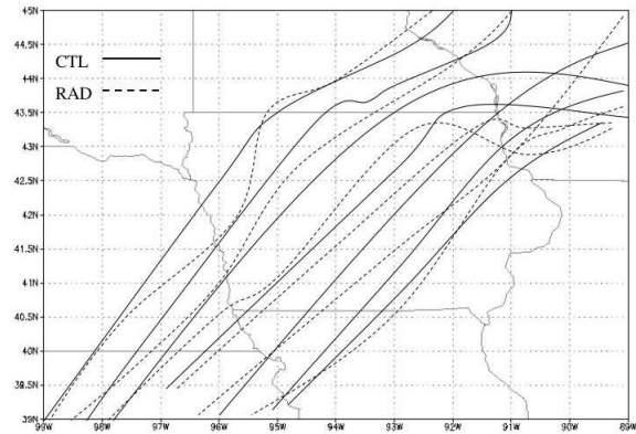
Figure 1: Frontal isochrone analysis from 12 Aug 2002 18 UTC to 13 Aug 2002 12 UTC. Solid line is CTL simulation and dashed line is RAD simulation.
