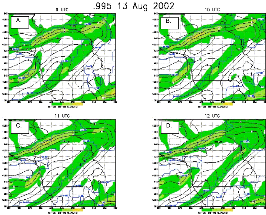
Figure 2: Gradient of potential temperature (shaded every 3 \times 10^{-5} from 3 \times 10^{-5} ), temperature difference between CTL and RAD (light solid positive, light dashed negative at 1K intervals) and Integrated cloud liquid water (dark contour of 0.00001 \text{ kg m}^{-3} ) at: A. 09 UTC B. 10 UTC C. 11 UTC D. 12 UTC..
