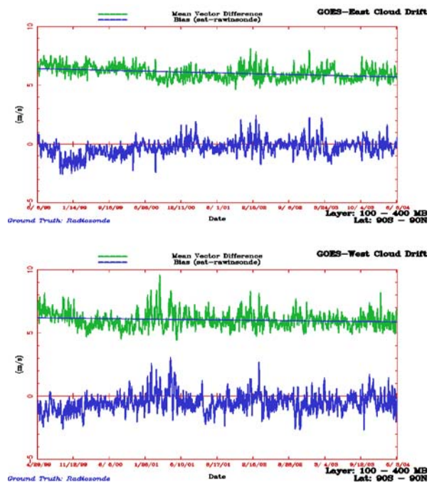
Figure 1. Mean vector difference and speed bias (sat-rawinsonde) for GOES-E (top) and GOES-W (bottom) upper level (100-400mb) IR cloud-drift winds.
