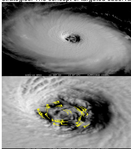
Figure 3. Hurricane Isabel in GOES-12 visible imagery on 12 September 2003 (top). Low-level AMVs in Isabel's eye derived from GOES-12 super-rapid scan (3-minute intervals used) visible imagery (bottom).
