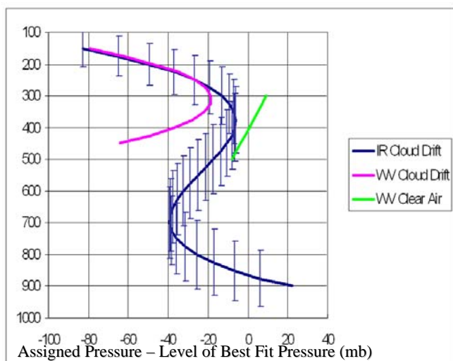
Figure 5. Height pressure difference (mb) profile (at every 25mb) between the assigned pressure and the level of best-fit pressure for GOES-8 IR cloud-drift, cloud-top water vapor, and clear-sky water vapor winds for the period Jan-Dec 2002. Error bars indicate one standard deviation about the mean difference values.
