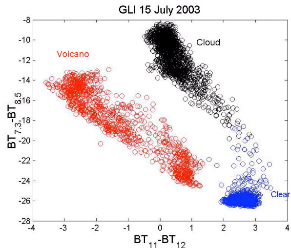
Figure 9: Japanese Global Imager data 11 – 12 um difference scene indicating the presence of volcanic ash. The 7.3 and 8.5 um differences provide a way to discriminate between volcanic ash, meteorological cloud and clear sky.
