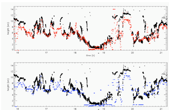
Figure 2: GOES-12 Imager (red) and Sounder (blue) cloud top height with CPL (black) cloud top height from the ATReC experiment.
