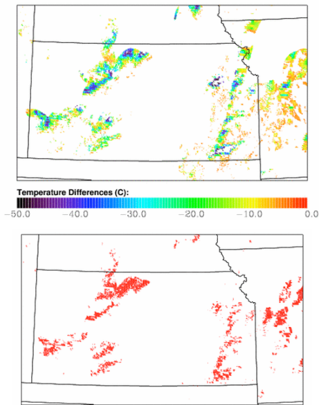
Figure 6: (top) 30-min cloud-top cooling rates for moving cumulus clouds using the AMVs shown in Figure 5. (bottom) The CI nowcast product. Pixels highlighted in red are cumulus where CI should occur 0-45 mins in the future.
