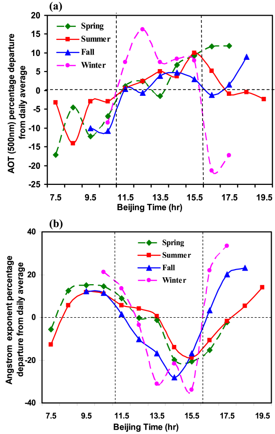
Figure 4: Diurnal variations expressed in terms of percentage departure from the daily mean for different seasons a) aerosol optical thickness at 500nm b) Angström exponent
