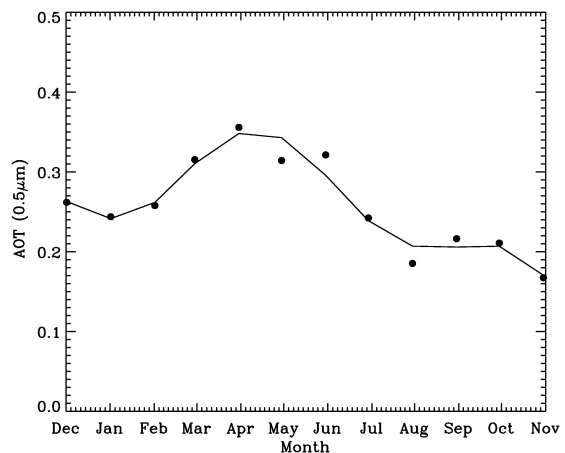
Figure 2: Monthly mean AOT (solid dots) in Dunhuang. The solid curve is the fit of AOT as a function of month ( m ): AOT = 0.52 - 0.11m - 1.07 \cos(2\pi(0.21m/12 - 0.29)) + 0.05 \sin(2\pi(1.09 - 1.84m/12)) . Note m starts from December, i.e., m=1 for December, m=2 for January and m=12 for November.
