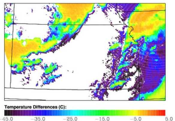
Figure 3: The 6.5–10.7 \mu\text{m} spectral band differencing technique at 2000 UTC on 4 May 2003.
