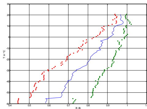
Figure 8 : Temperature versus ratio of intensity R/B obtained from 1400000 measures.
