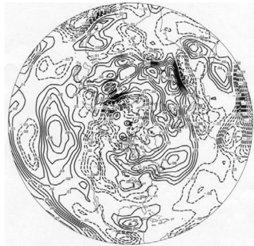
Figure 1. The u-wind component mean wind speed trend 1951 - 2000.
