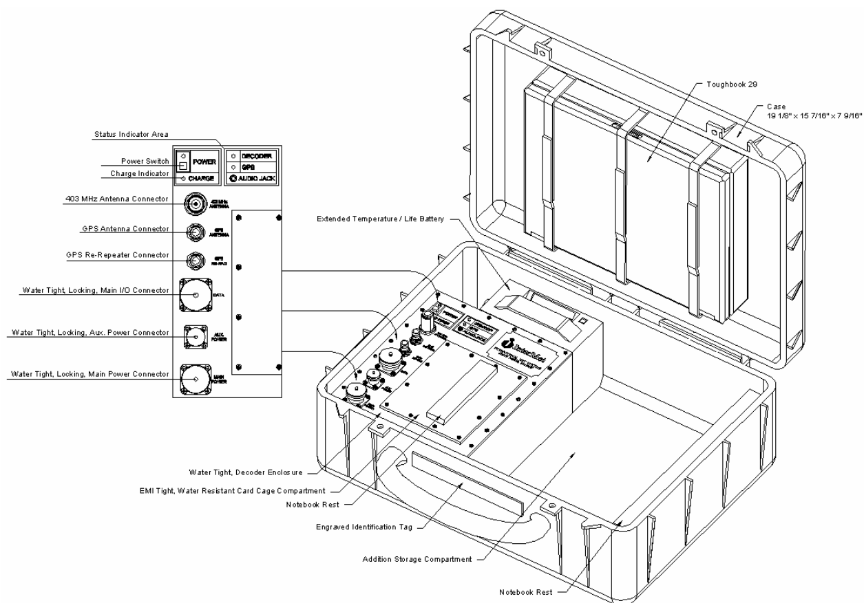
Figure 3: Portable 403 MHz Radiosonde System Ground Station
