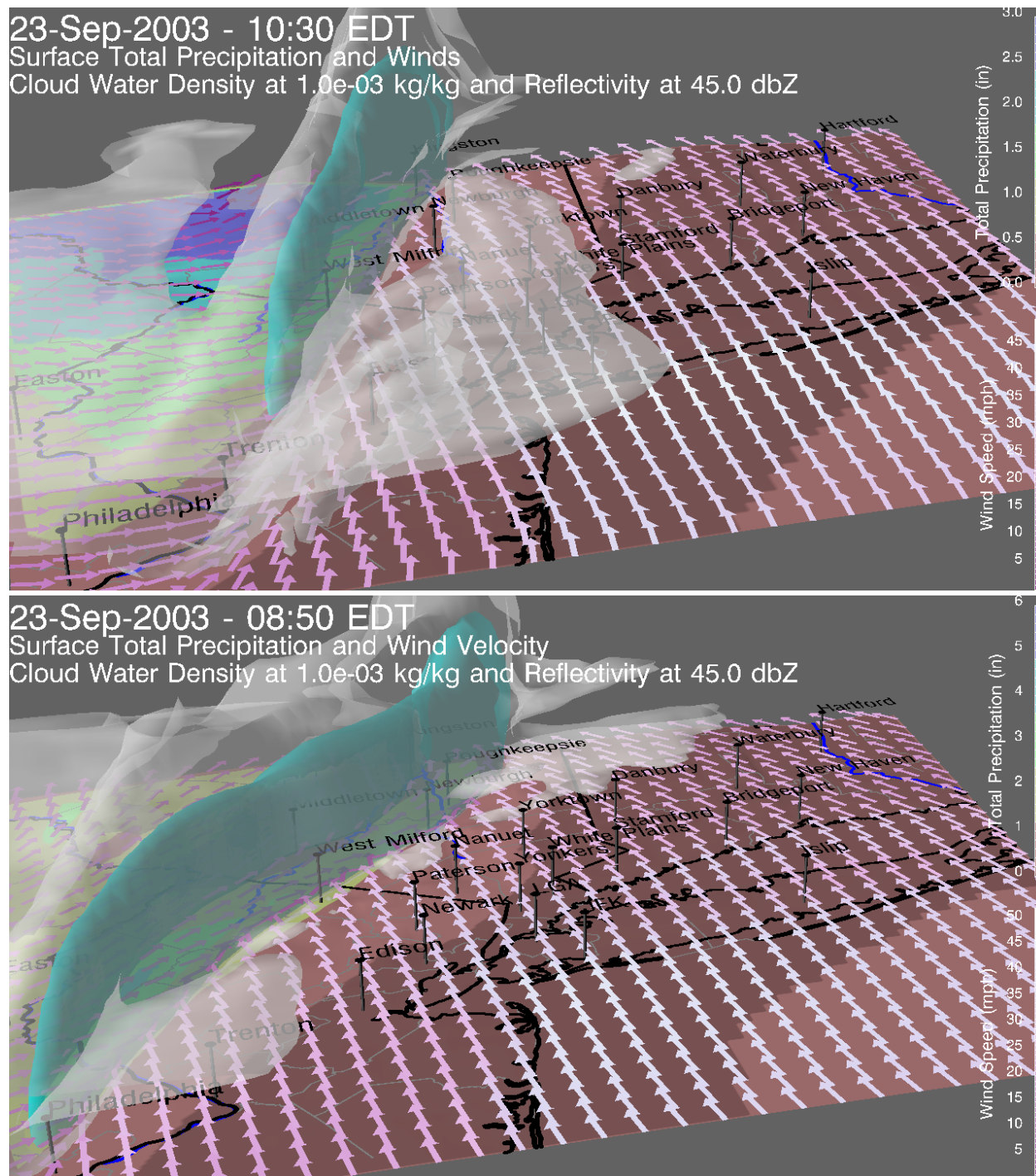
Figure 4. Deep Thunder Forecasts of Severe Thunderstorm Event of September 23, 2003.
